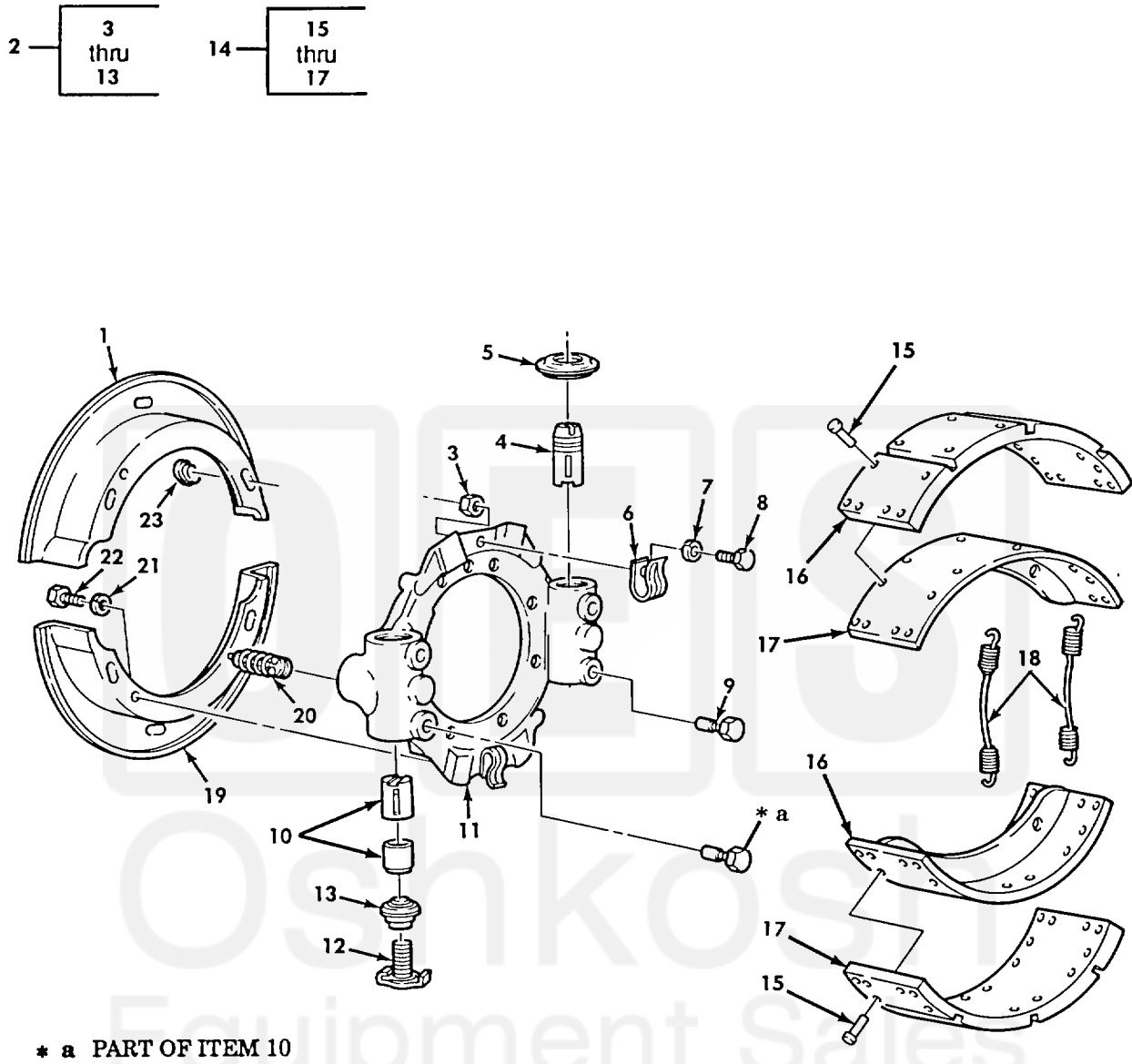
Figure 245. Front Axle Brake and Spider Assembly.
